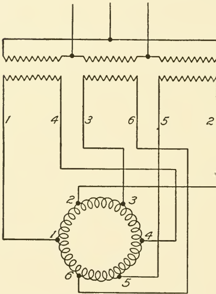
Fig. 33. Transformer Connections from Three Phase to Six-Phase for Rotary Converter
